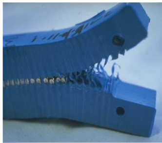
FIGURE 4 – DUCTILE BEHAVIOUR
