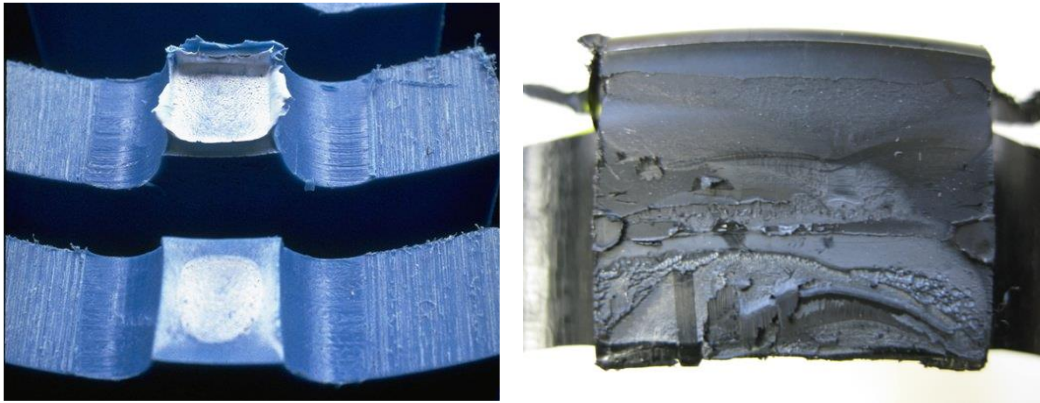
FIGURE 3 – SHOWING “MIXED” AND BRITTLE FAILURE MODES OF TENSILE SPECIMENS
