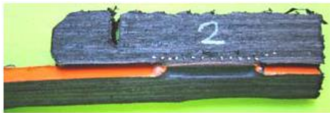
FIGURE 7 – ISO 21751 STRIP BEND TEST SHOWING ACCEPTABLE EF WELD AFTER BEND TESTING
