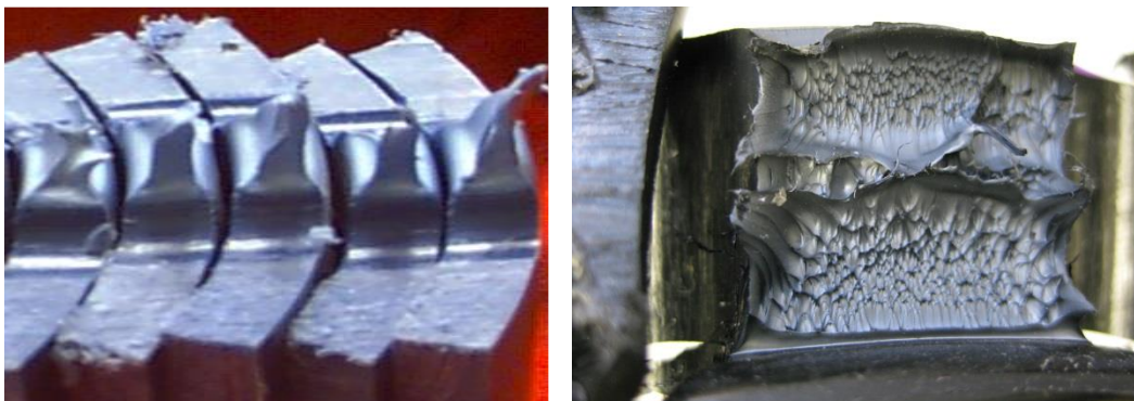
FIGURE 2 – SHOWING FULLY DUCTILE FAILURE MODE OF TENSILE WELD SPECIMENS
