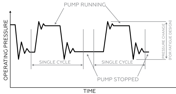
Figure 1.3 Inputs for fatigue design – pressure amplitude and frequency
