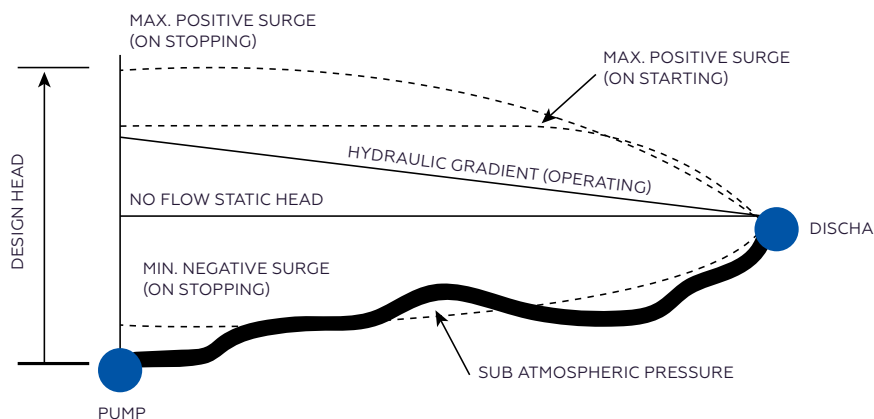
Figure 1.0 Typical hydraulic grades and surge envelopes required for design of Rhino ® PVC-M Pipe
